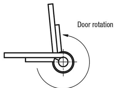
Hinges with opening spring
