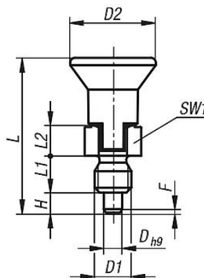
Form C lockout type without locknut
